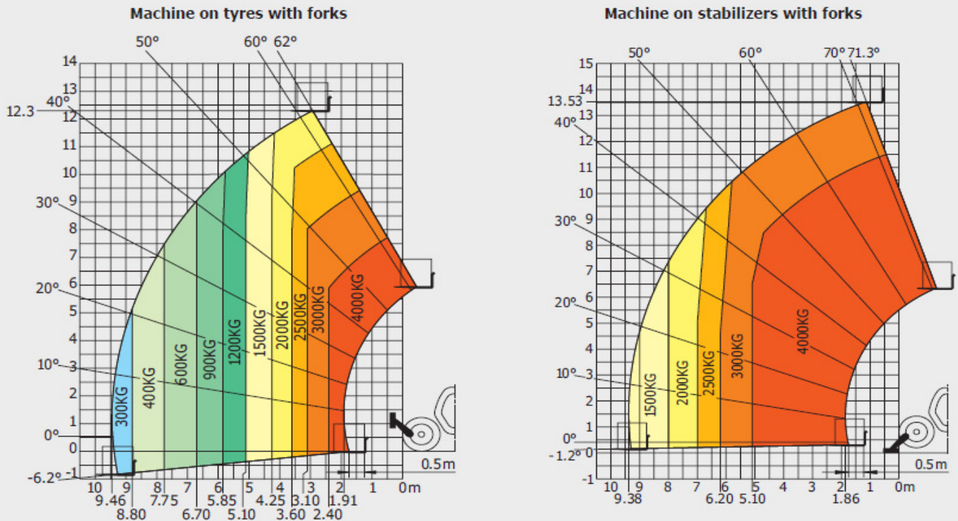
Rough terrain load chart standard EN1459 B
